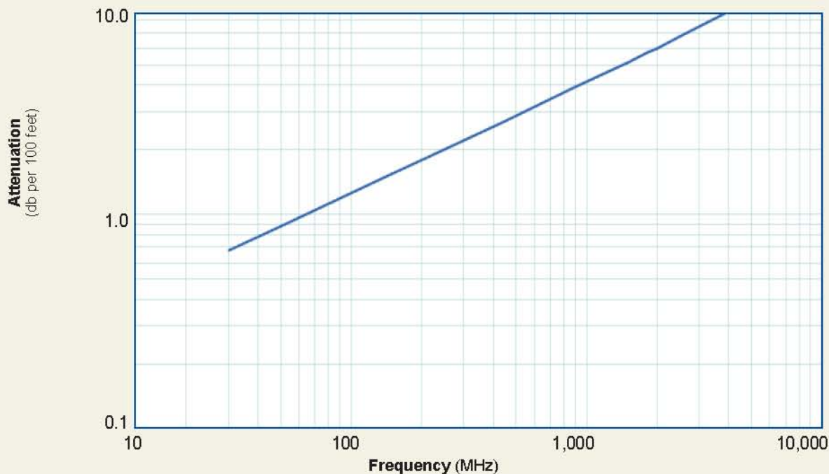
Attenuation vs. Frequency (typical)
