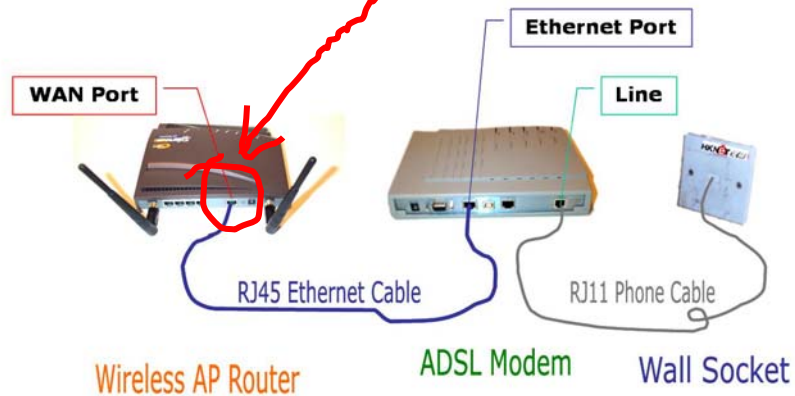
STEP 2 - Plug it straight into the WAN Port of the wireless AP Router. You don't have to remove any cables at the HKNet's ADSL Modem and the Wall Socket
